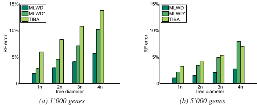
Fig. 5. RF error rates for different approaches for trees with 100 species, with genomes of 1'000 and 5'000 genes and tree diameters from one to four times the number of genes, under the rearrangement model.
