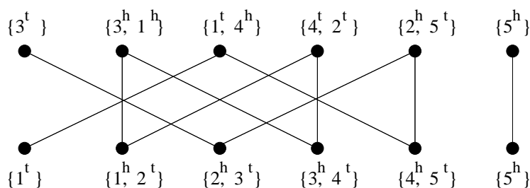
Fig. 2. Adjacency graph and DCJ distance of two genomes G_1 = (3, -1, -4, 2, 5) and G_2 = (1, 2, 3, 4, 5) . The number of cycles C is 1, the number of odd paths I is 2, the DCJ distance is N - (C + I/2) = 3 .
