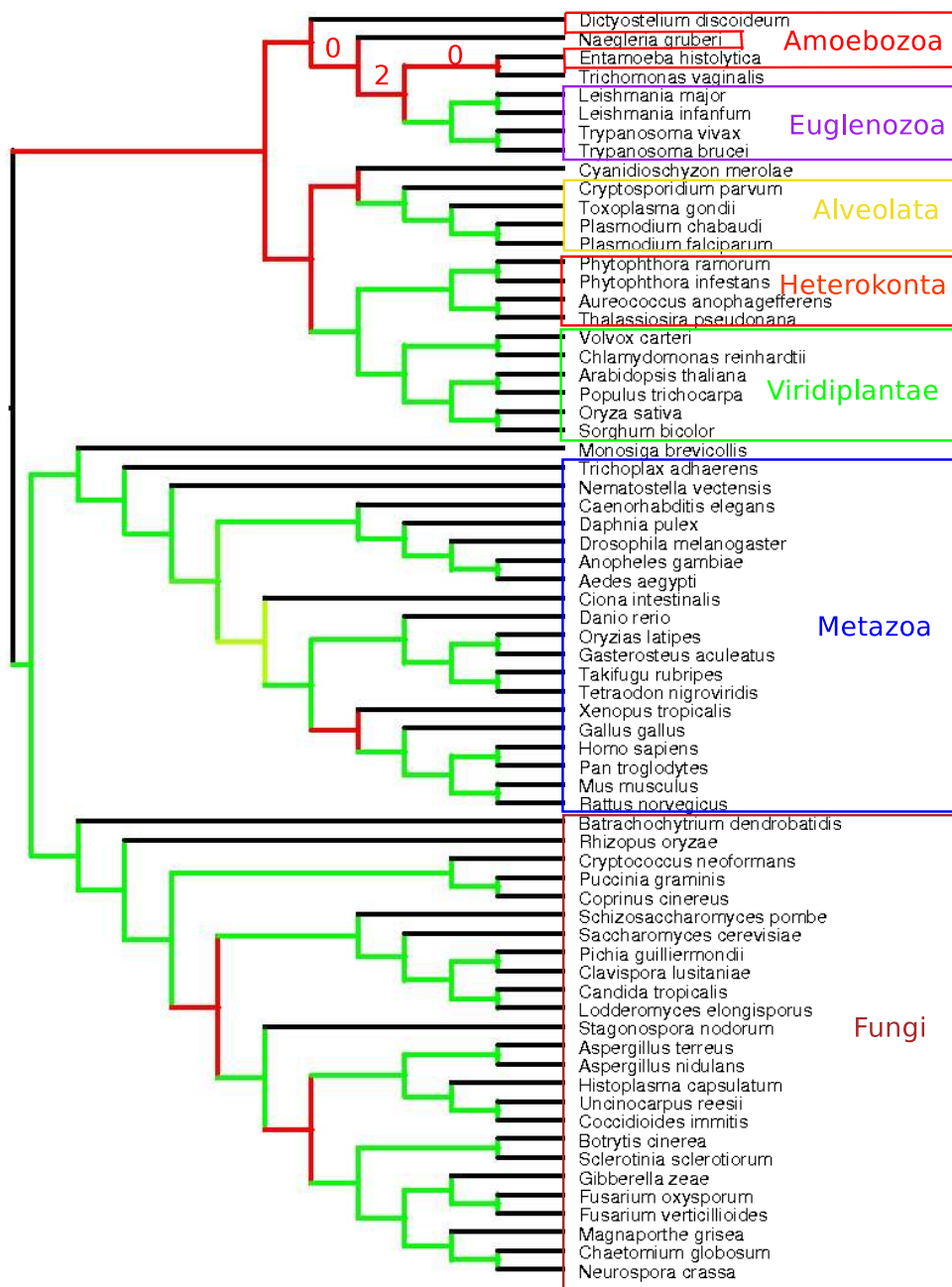
Fig. 6. The inferred phylogeny of 68 eukaryotic genomes, drawn with iTOL [40]. Internal branches are colored green, yellow, and red, to indicate, respectively, strong (bootstrap value > 90), medium (bootstrap value between 60 and 90), and weak support (bootstrap value < 60).
