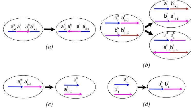
Fig. 3. Possible rearrangements in the HP model: (a) inversion, (b) translocation, (c) fission, and (d) fusion.
